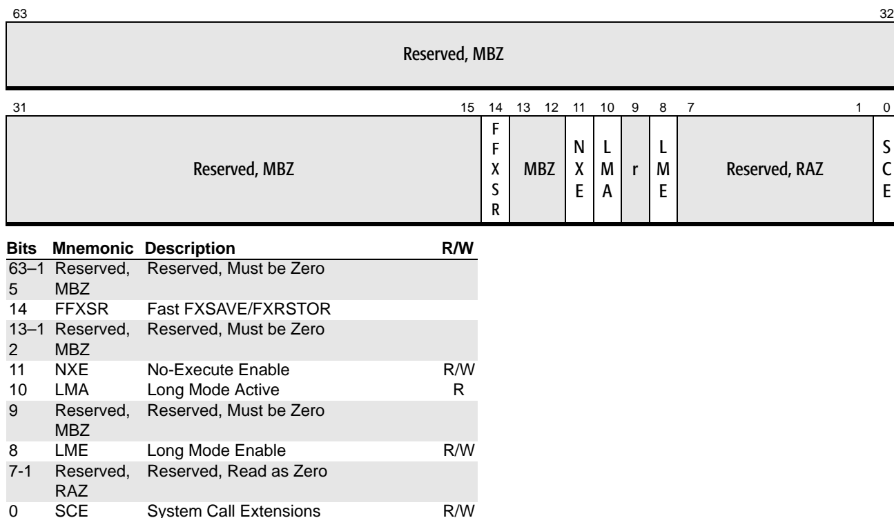
Figure 3-9. Extended Feature Enable Register (EFER)
