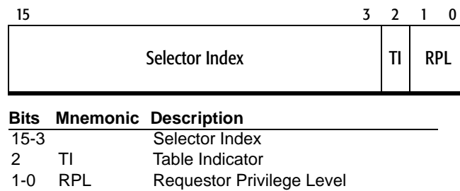
Figure 12-2. Task-Segment Selector
