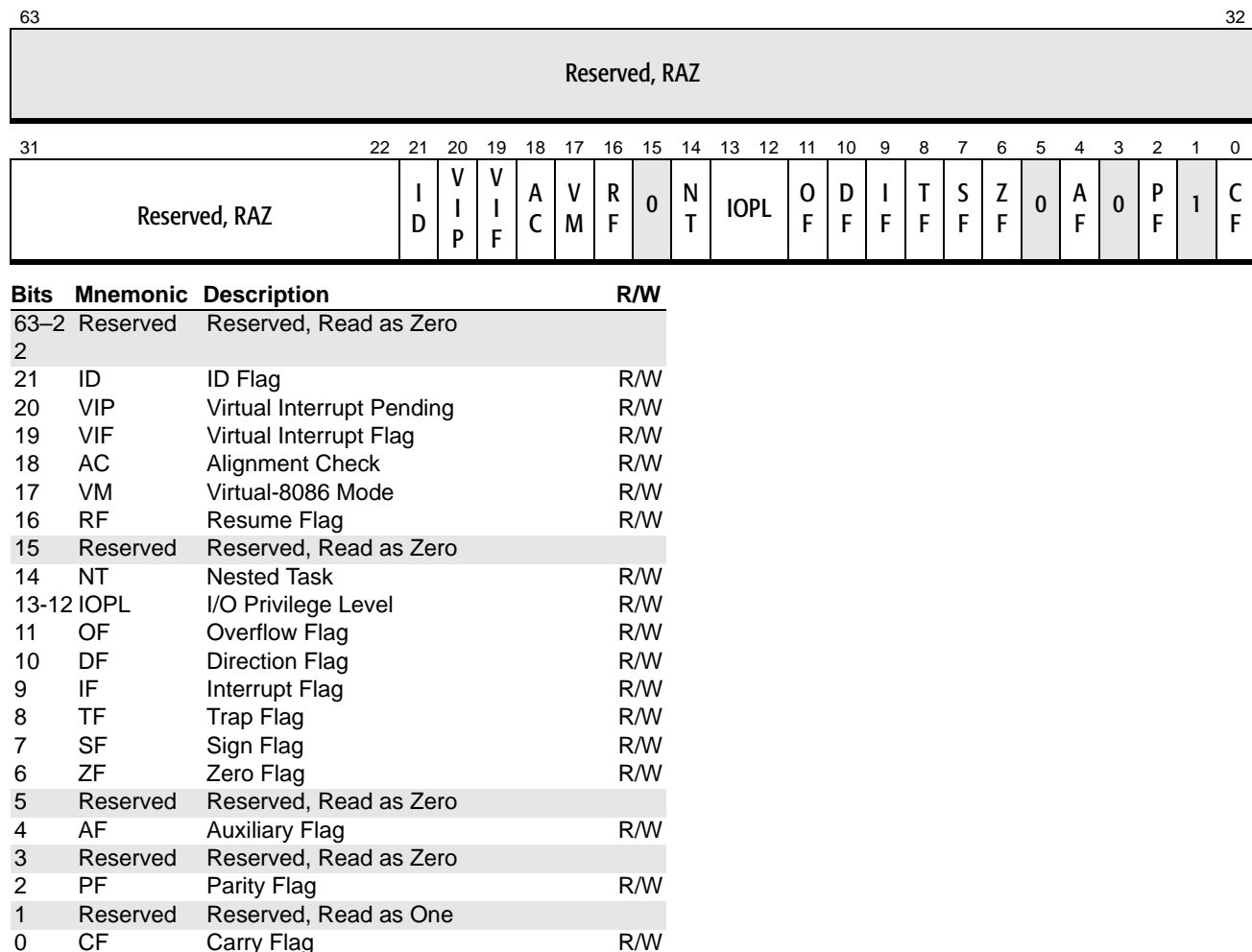
Figure 3-8. RFLAGS Register
