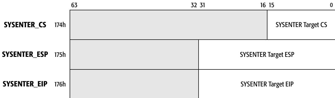
Figure 6-2. SYSENTER_CS, SYSENTER_ESP, SYSENTER_EIP MSRs
