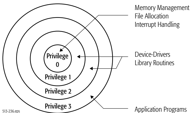
Figure 4-25. Privilege-Level Relationships
